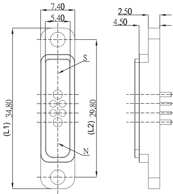
Dimension Table From 4 Pin to 16 Pin
