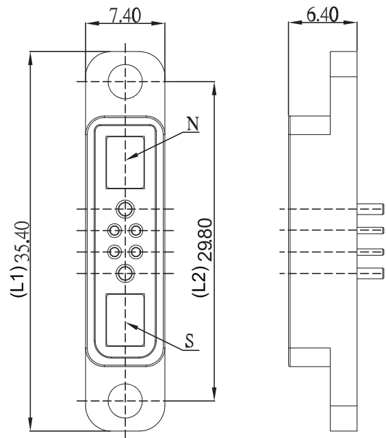
Dimension Table From 4 Pin to 16 Pin
